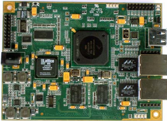
Topside View
